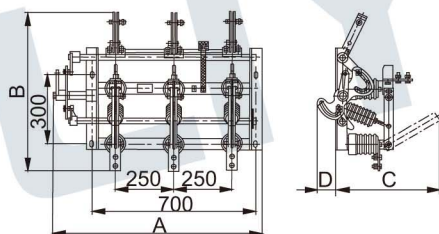
Diagram 3 GN24-12D II
