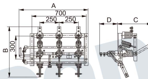
Diagram 2 GN24-12DC I
