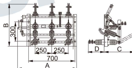
Diagram 4 GN24-12DC II
