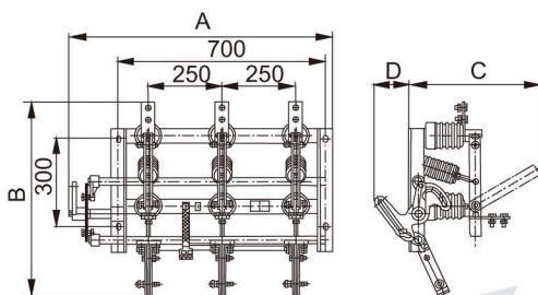
Diagram 1 GN24-12D I
